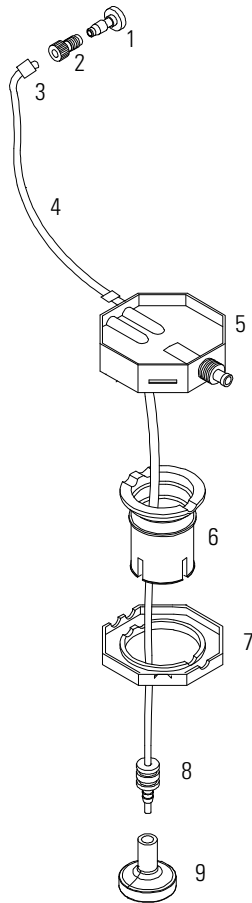
Figure 30 Bottle-Head Assembly Parts
